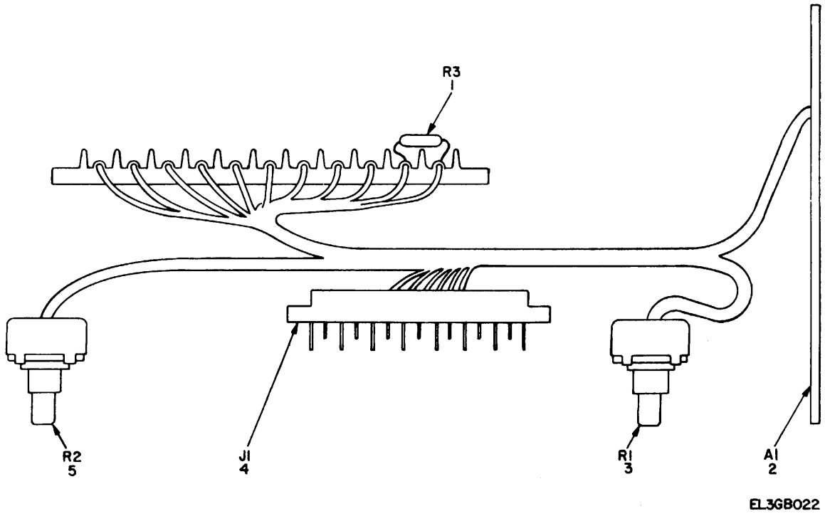
Figure 20. Wiring Harness A2W1.
