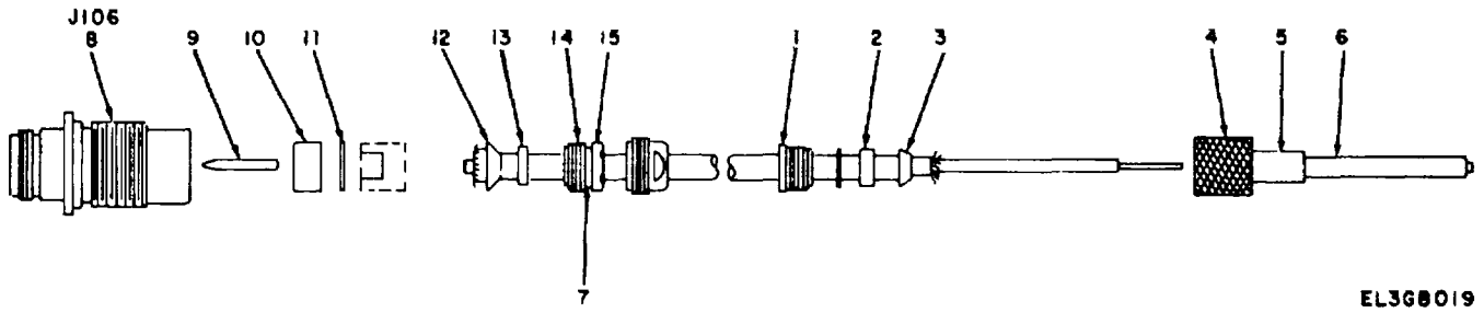
Figure 17 . Probe Assembly A2A3 .
