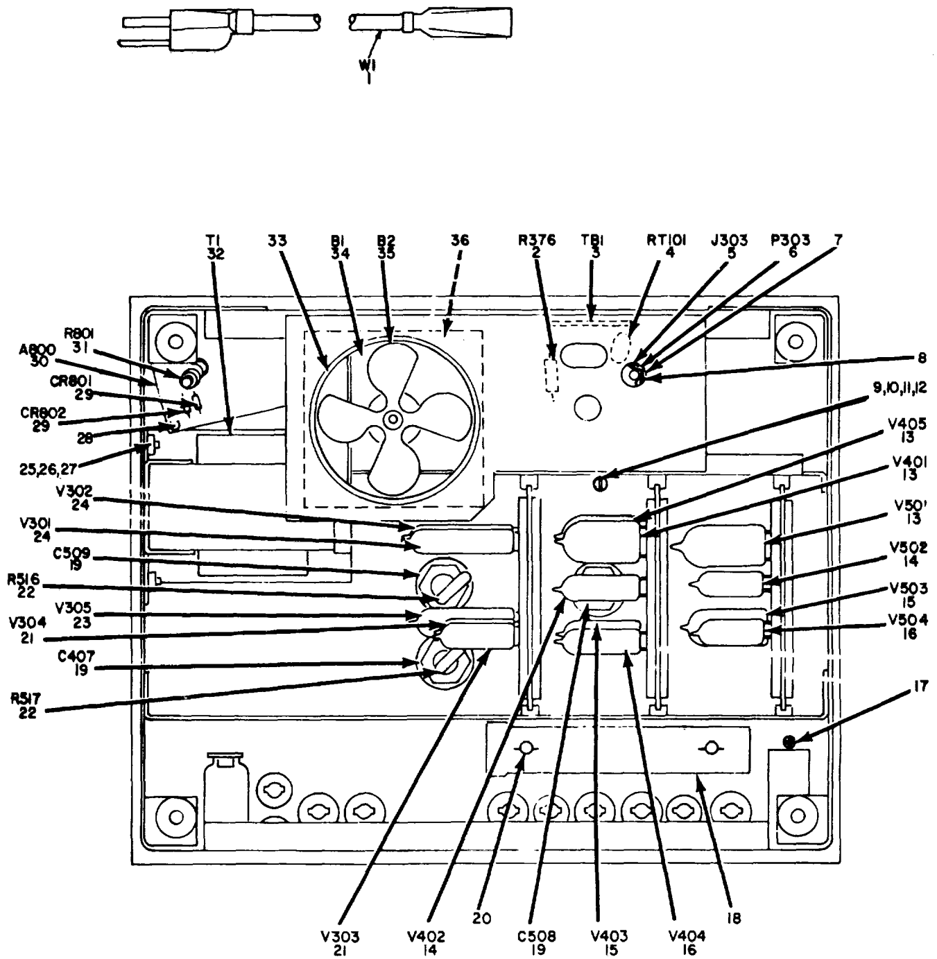
Figure 2. Signal Generator SG-756/URM, Rear View Cover and Power Cable Removed.
