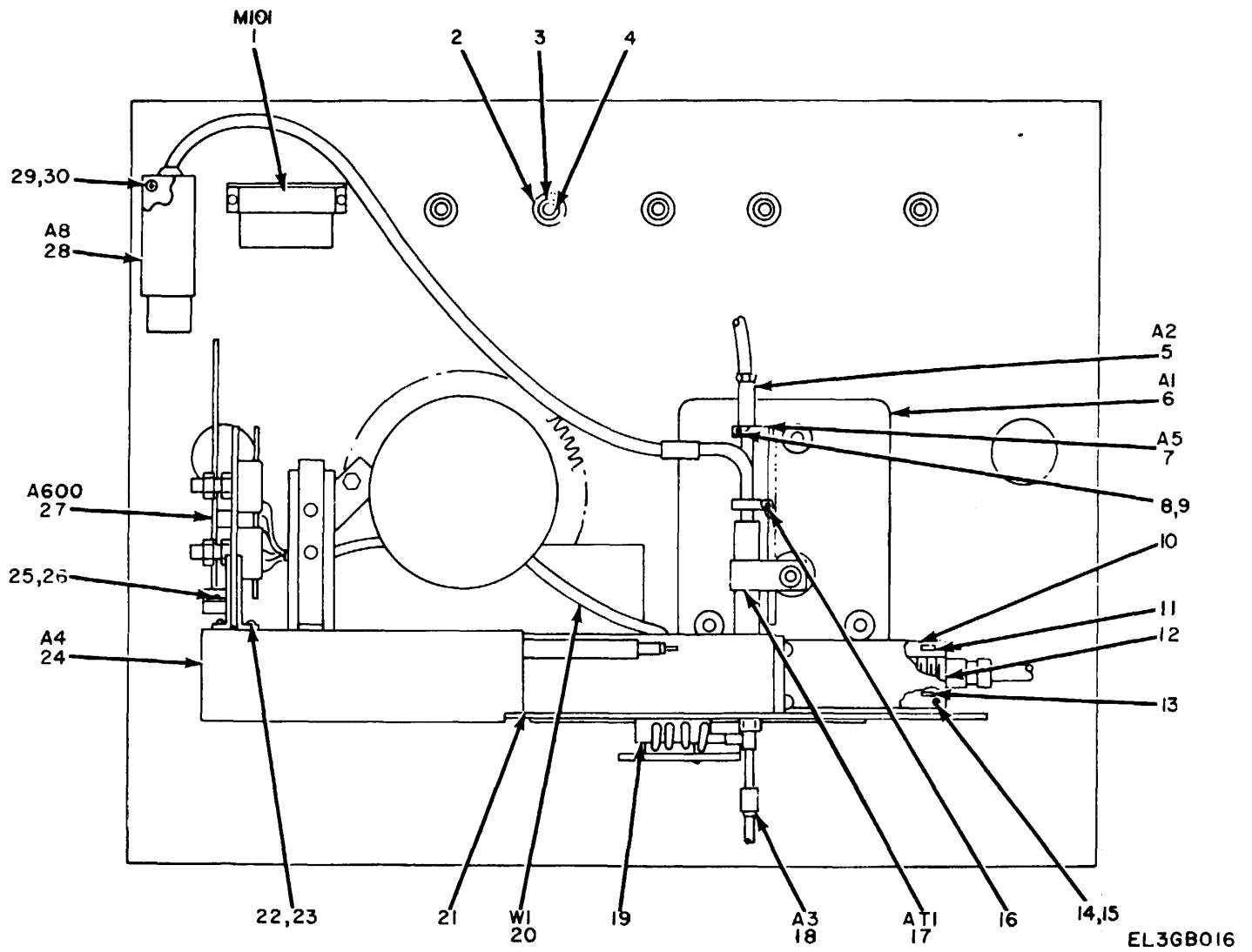
Figure 14. Front Panel Assembly, Rear View .
