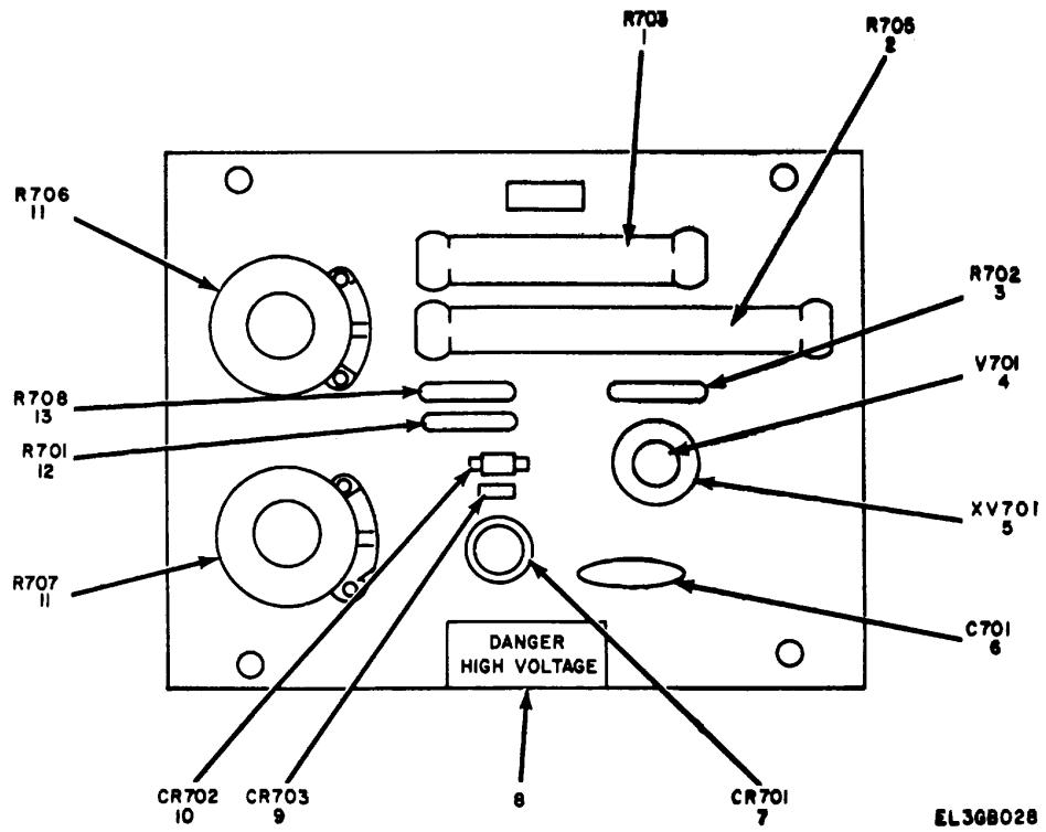
Figure 26. Circuit Card Assembly A700.
