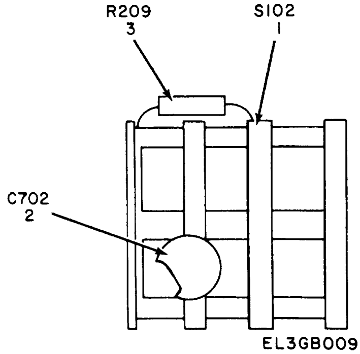
Figure 9. Switch Assembly, Rotary AA11 .
