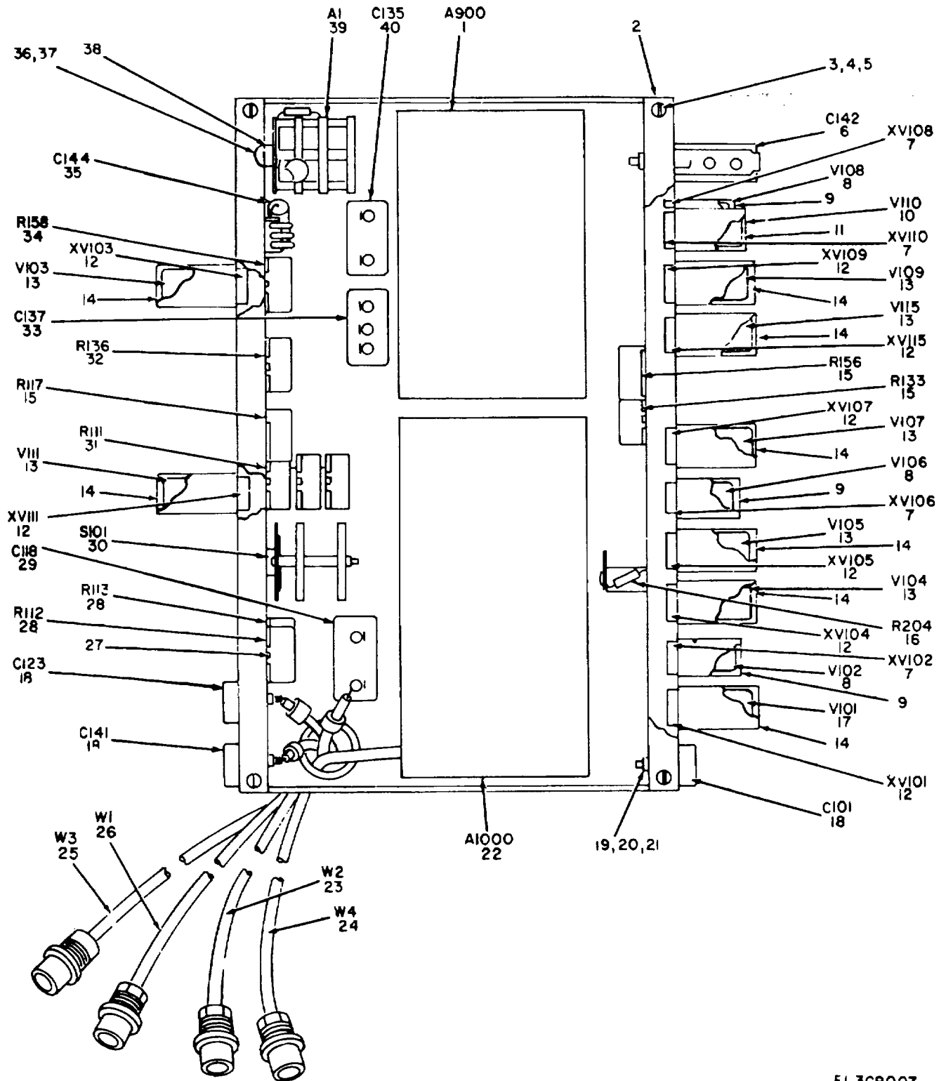
Figure 7. Pulsar Assembly A1 .
