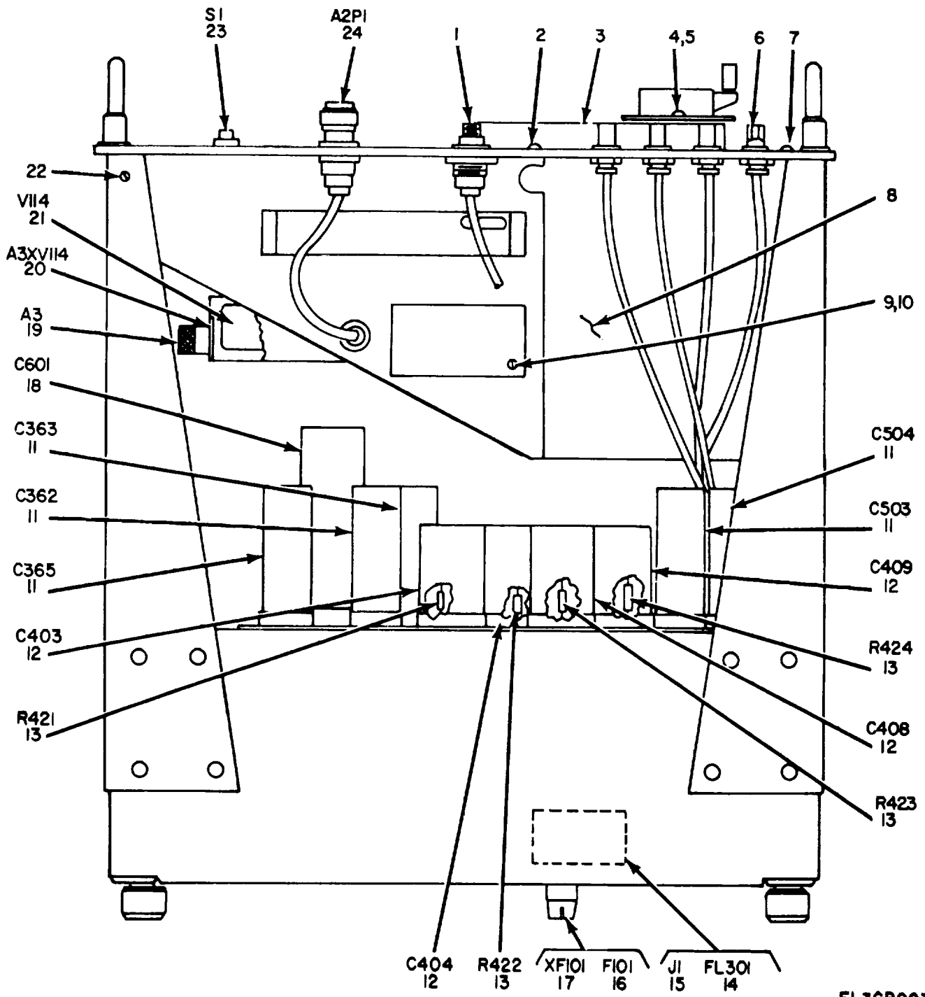
Figure 3. Signal Generator SG-756/URM, Bottom View, Cover Removed.
