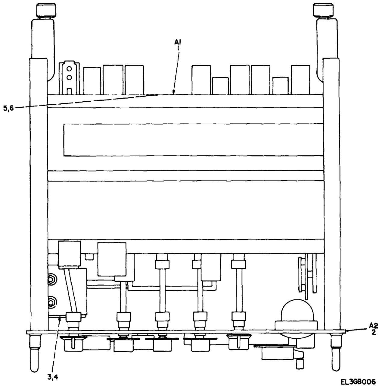
Figure 6. Signal Generator SG-756/URM, Top View, Cover Removed .
