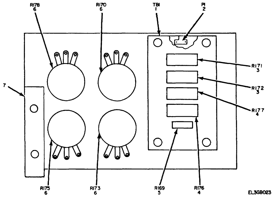
Figure 21. Resistor Board Assembly A2W11A1.
