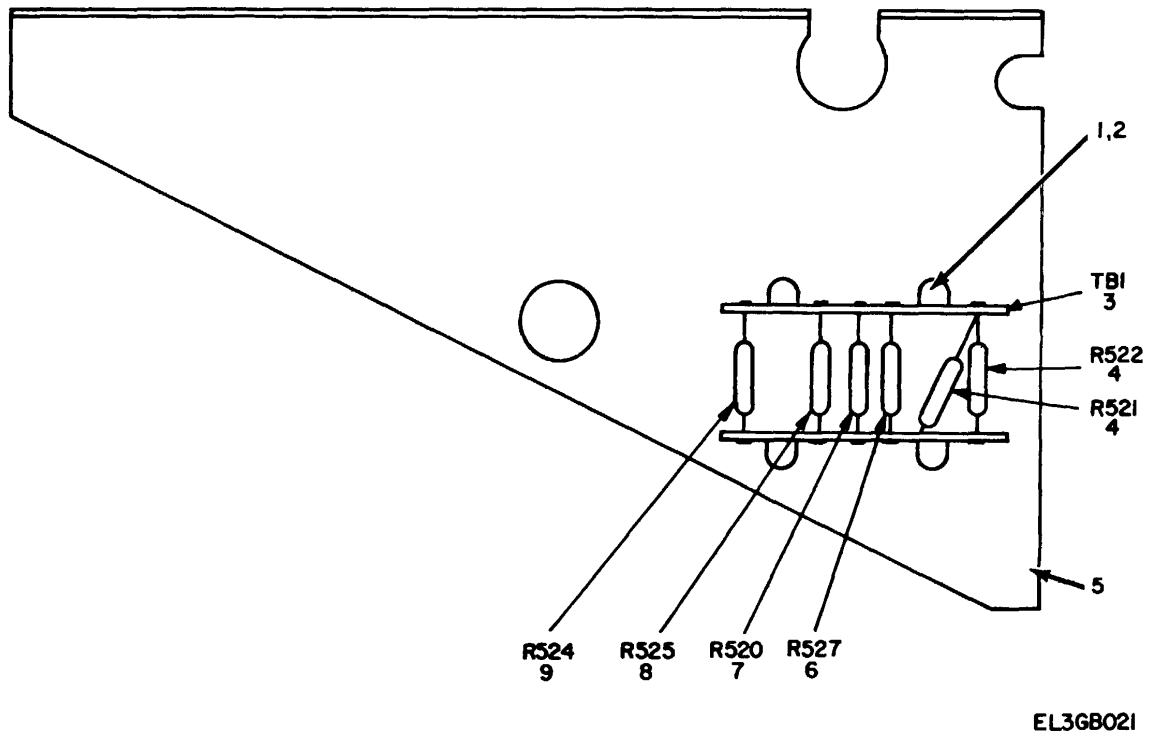
Figure 19. Divider Assembly A2AS.
