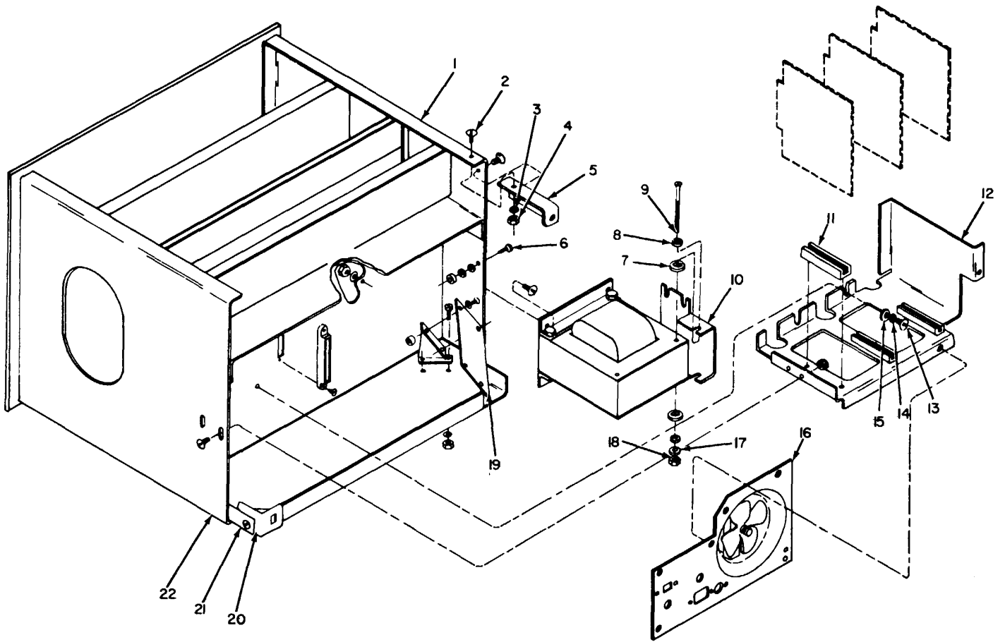
Figure 4. Signal Generator SG-756/URM, Chassis, Rear View .
