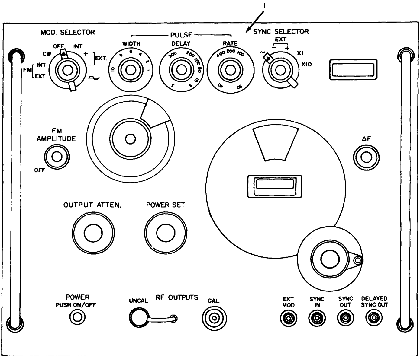
Figure 1. Signal Generator AN/URM-170 .
