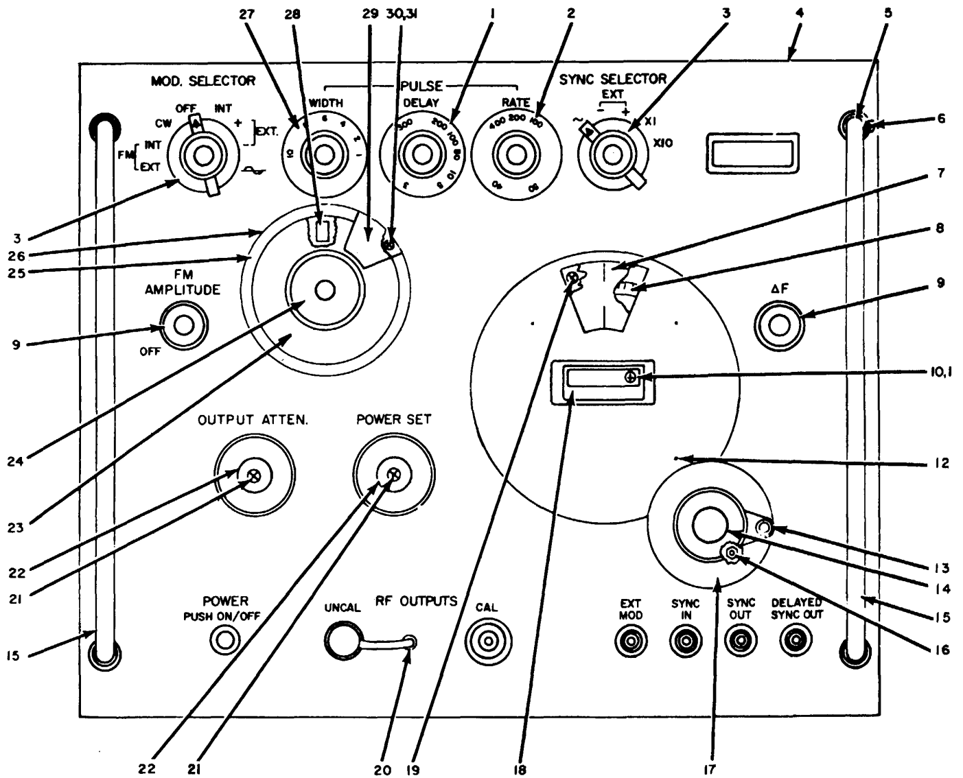
Figure 13. Front Panel Assembly, Front View .
