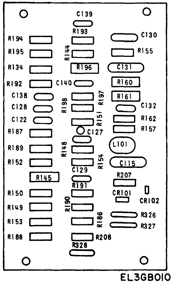
Figure 10. Circuit Card Assembly A1A900 (Sheet 1 of 2).
