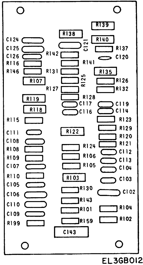
Figure 11. Circuit Card Assembly A1A1000 (Sheet 1 of 2).
