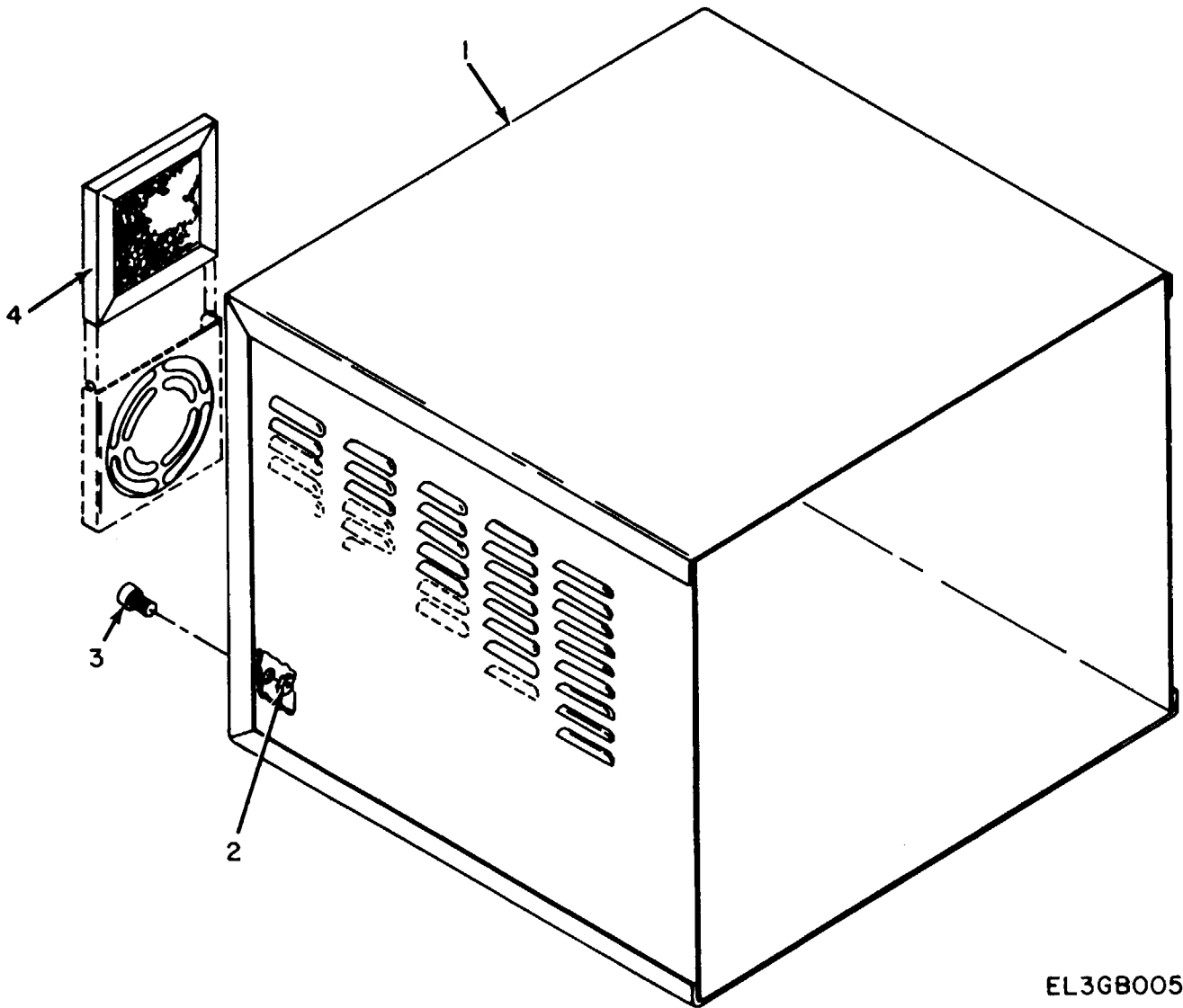
Figure 5. Signal Generator SG-756/URW, Dust Cover .
