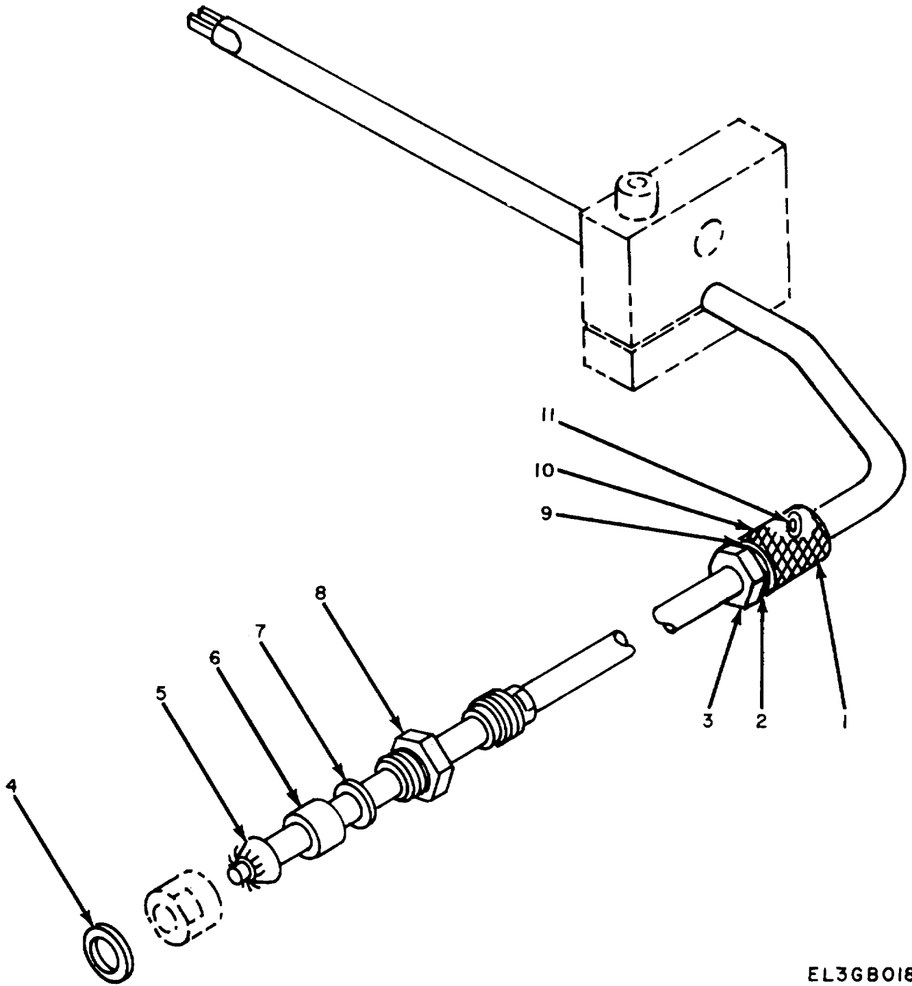
Figure 16. Probe Assembly A2A2 .
