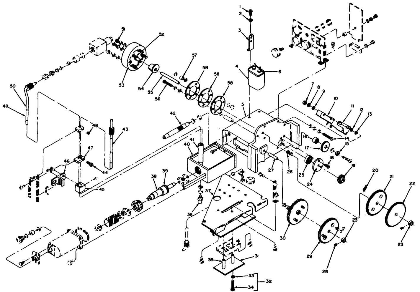
Figure 18. Frequency Control Assembly A2A4.
