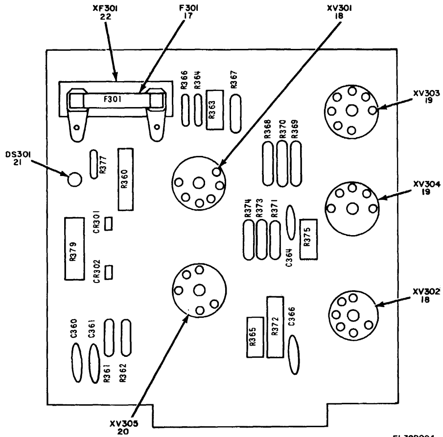
Figure 22. Circuit Card Assembly A300.
